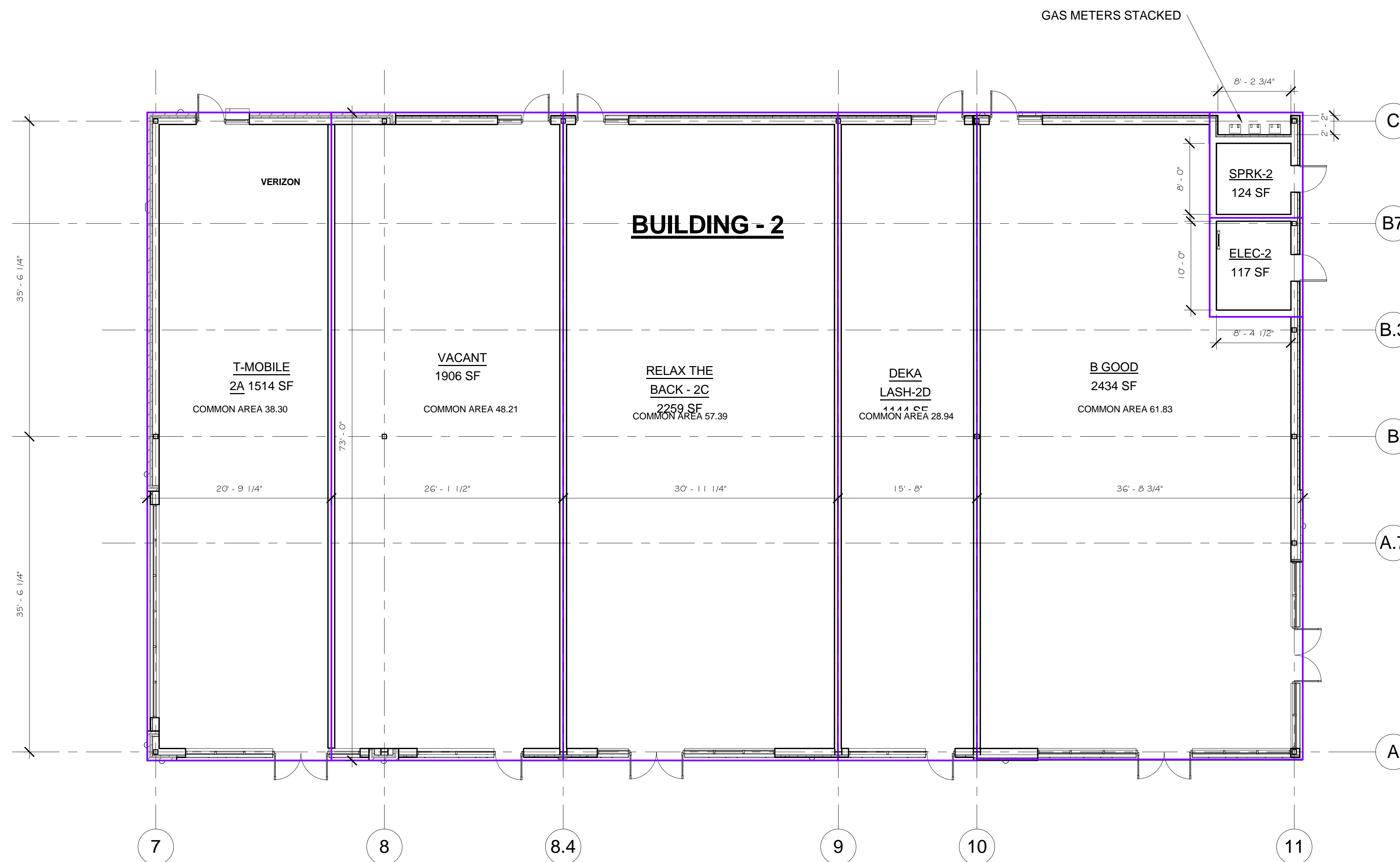
1 FIRST FLOOR LOD BUILDING 2 1/8" = 1'-0"
